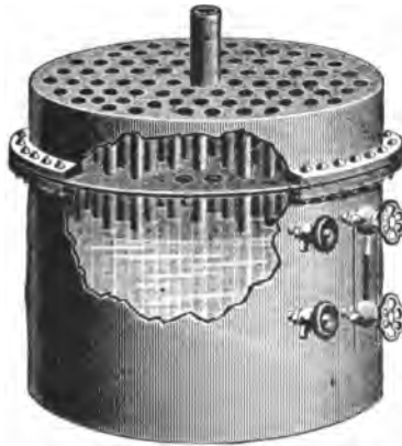
FIG. 124.—The Kitts-Tonkin Dry-Plate Boiler, for steam carriages. This boiler consists of two seamless steel pressings riveted together through a flange, as shown. The flues are inserted through perforations in the upper and lower crown sheets, and in the intermediate dry plate, also secured by the rivets. Sufficient space is left around the flues to allow the steam to collect above the plate, going thence to the engine. The dry plate forms a very efficient separator. The steam connection to the engine is by the vertical tube at the centre of the upper tube plate. It extends only a short distance into the space above the dry plate, thus ensuring the feeding of perfectly dry steam.
